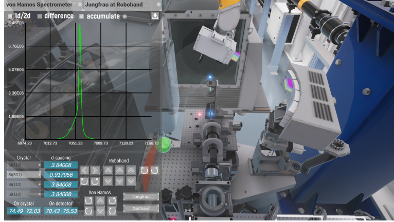
Figure 8: The Vonamos spectrometer in operating position. with the read-out of the Jungfrau detector as well as the settings for the position to the left.
