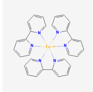
Figure 2: Schematic view of [Fe(bipy)_3]^{2+}
