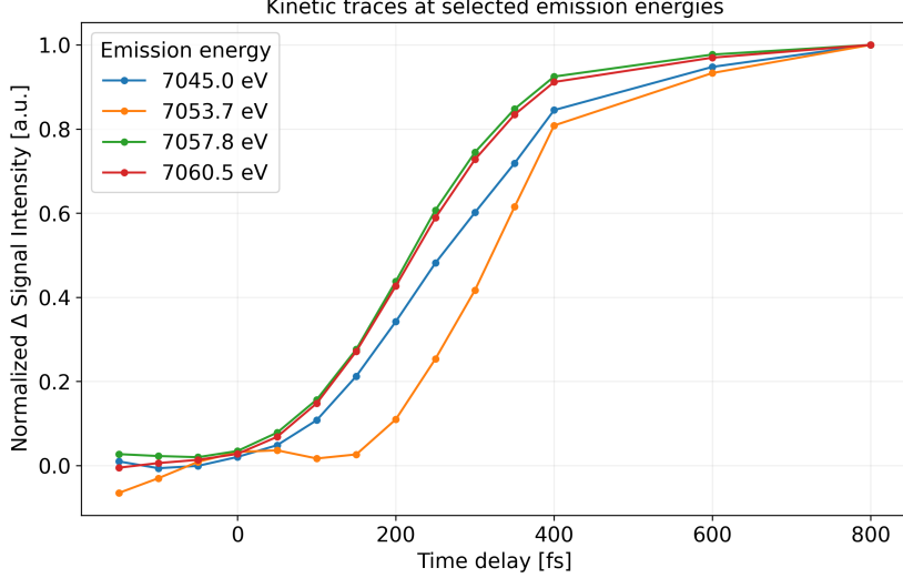
Figure 12: Kinetic traces at selected emission energies.
