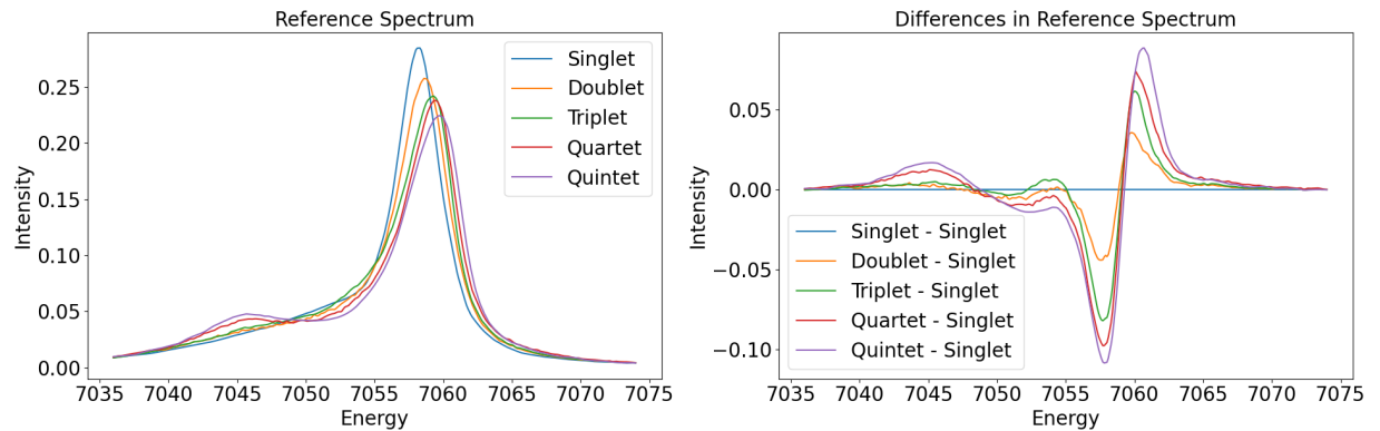
Figure 9: The reference spectra plotted with provided data for different spin states. The reference difference spectra with transient signals plotted with provided data for different transitions.
