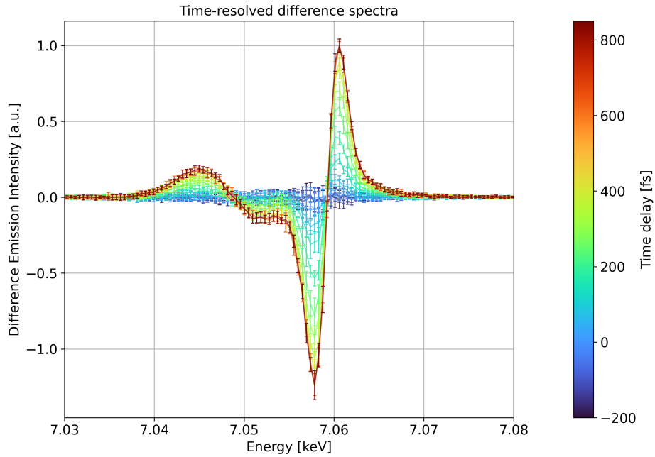
Figure 11: Transient spectra of the X-ray emission at different pump-probe time delays.
