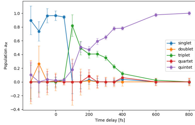
Figure 16: The adjusted population curves of the different spin states plotted against the time delay of the optical laser in femtoseconds.
