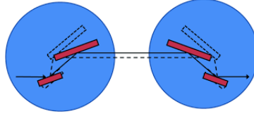
Figure 3: Optical layout of a four-crystal monochromator [?].
