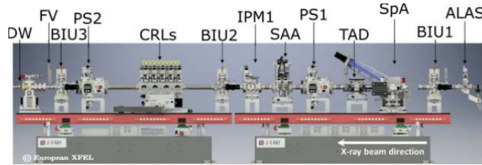
Figure 4: The optical bench in the FXE hut with the following components implemented: BIU 1,2,3 (beam imaging units), SpA (spectrum analyser), TAD (time arrival detector), PS 1,2 (power slits), SAA (solid attenuator assembly), IPM1 (intensity position monitor), CRLs (compound refractive lenses) [4].
