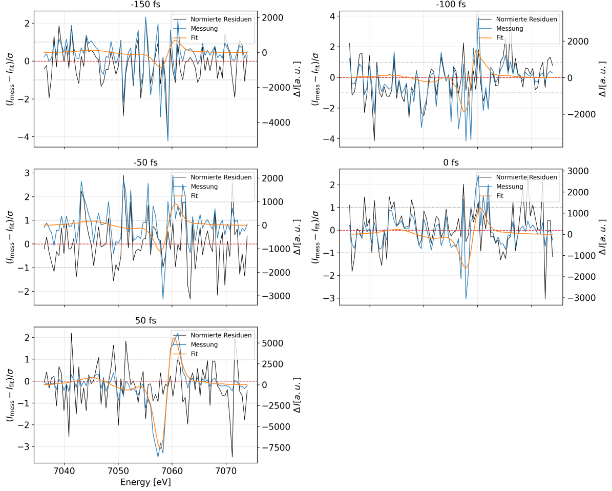
Figure 14: The normalised residuals together with the actual measurements and a fit over ... for time delays of \Delta t = \{-150 \text{ fs}, -100 \text{ fs}, -50 \text{ fs}, 0 \text{ fs}, 50 \text{ fs}\}
