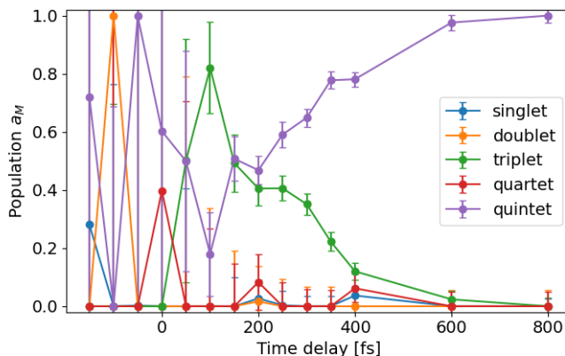
Figure 13: The population curves of the different spin states plotted against the time delay of the optical laser in femtoseconds.
